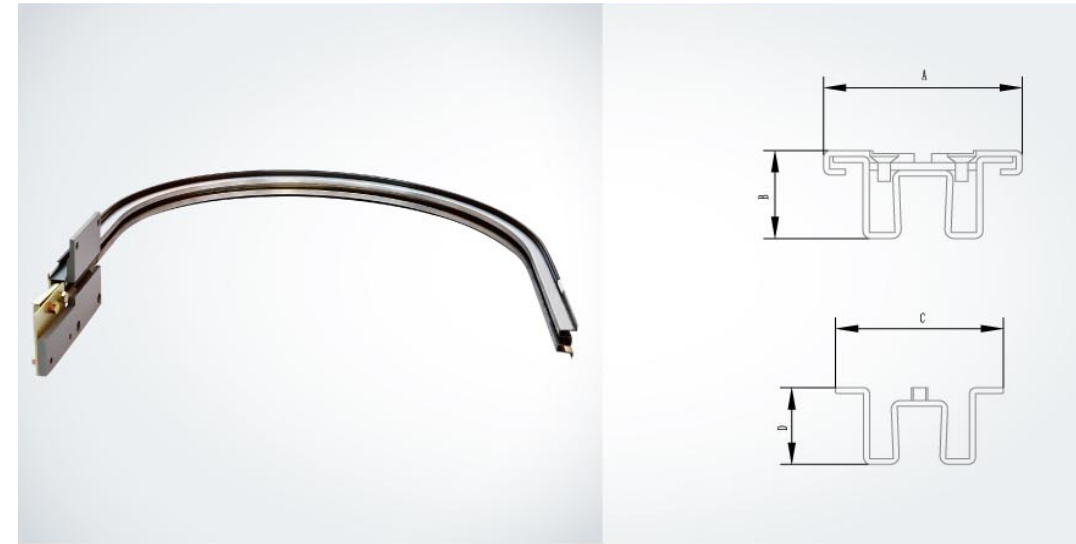
扶手转角栏杆 Balustrade header
