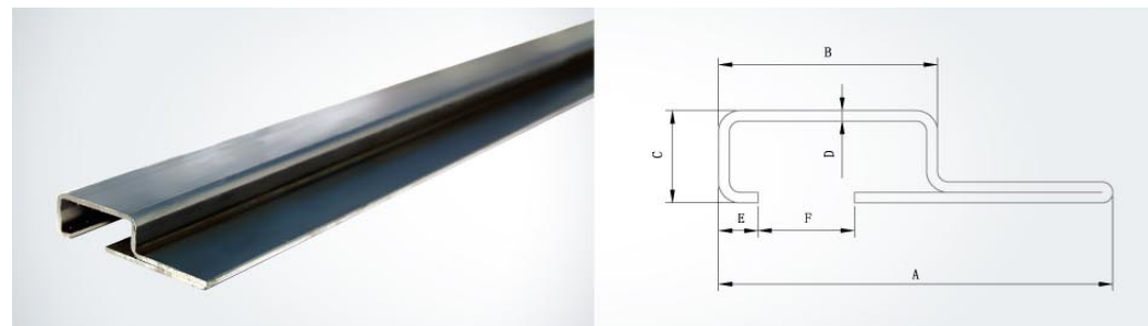
回路随动导轨 Secondary counter rail
