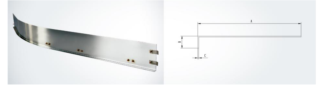
弯曲围裙板 Curving skirting plate
