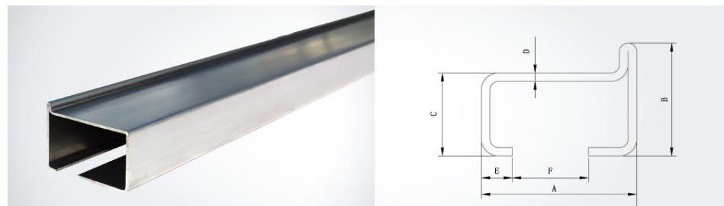
回路驱动导轨 Driving counter rail
