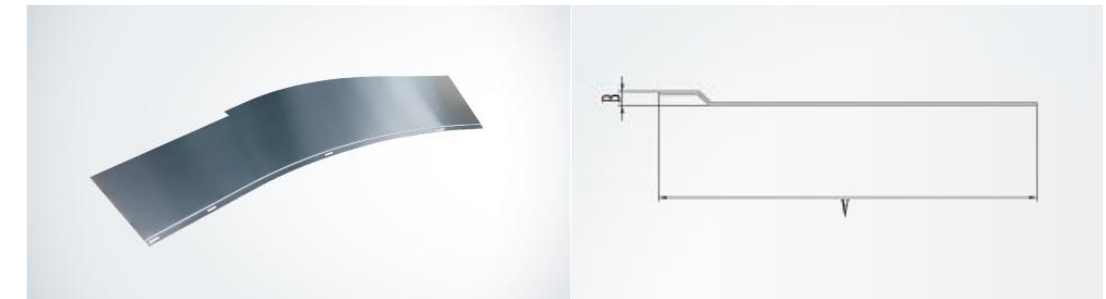
内盖板 Curving interior panel
